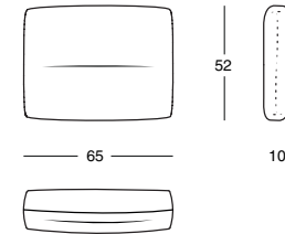
1338/65C
